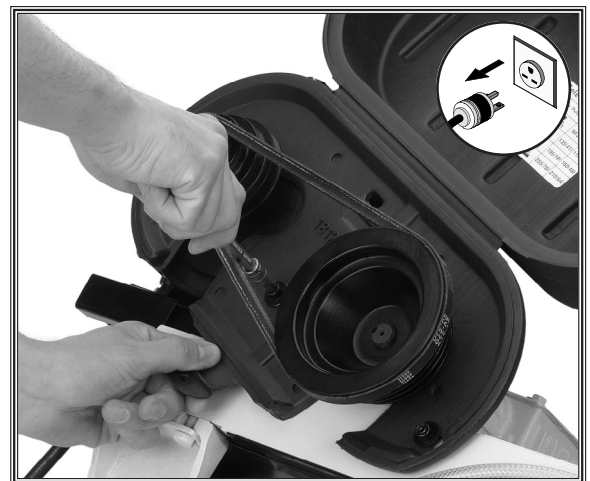
Figure 20. Securing the pulley cover.
